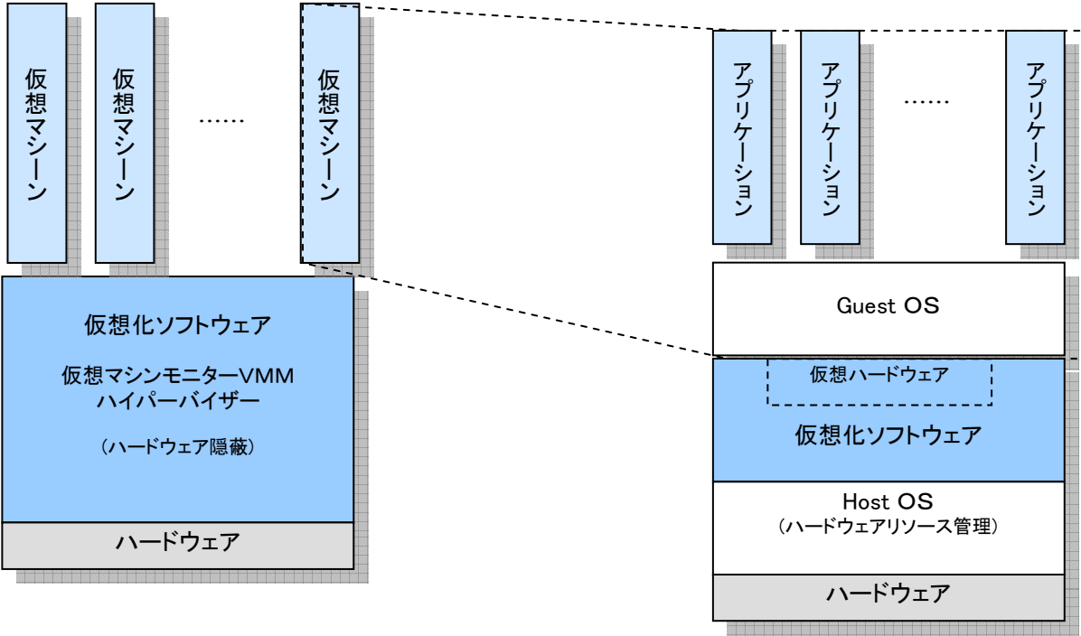
Basic Architecture
